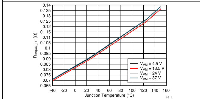
Figure 6. Low-Side R_{DS(on)} vs. Junction Temperature
