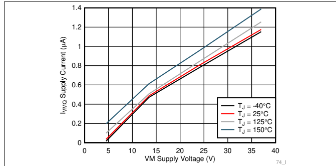
Figure 2. Sleep Current ( I_{VM0} ) vs. Supply Voltage ( V_{VM} )
