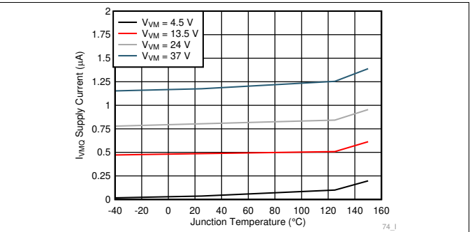
Figure 3. Sleep Current ( I_{VM0} ) vs. Junction Temperature
