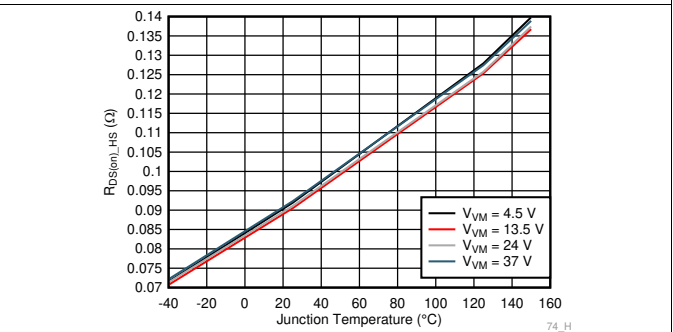
Figure 7. High-Side R_{DS(on)} vs. Junction Temperature
